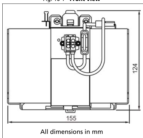
Fig. 16-1 Front view
