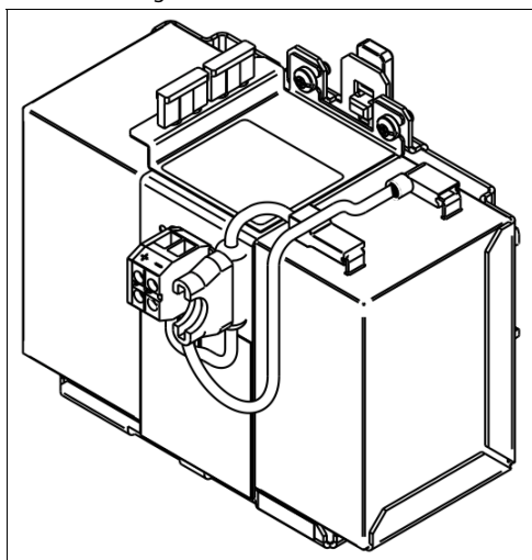
Fig. 16-3 Isometric view
