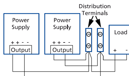
Fig. 13-2: Using distribution terminals
