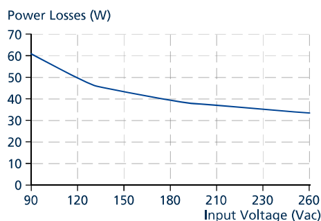
Fig. 9-4: Losses vs. input voltage at 24 V, 40 A, typ.
