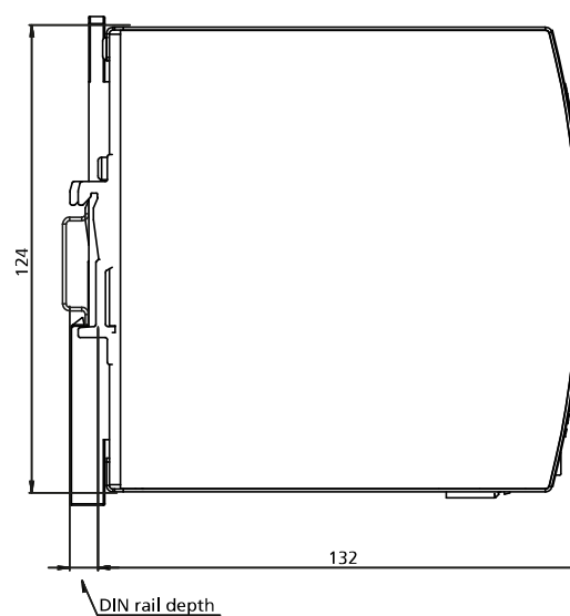
Fig. 22-2: Side view
