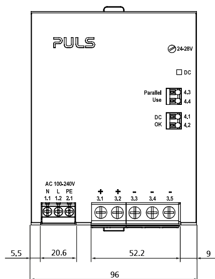
Fig. 22-1: Front view
