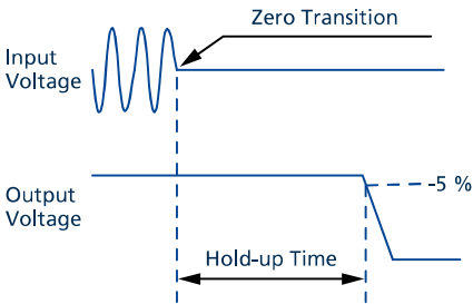
Fig. 7-2: Shut-down behaviour
