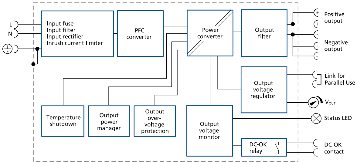
Fig. 12-1: Functional Diagram SP960.241-S
