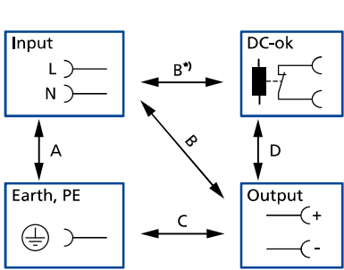
Fig. 19-1: Dielectric strength
