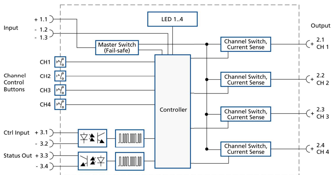
Fig. 12-1: Functional diagram
