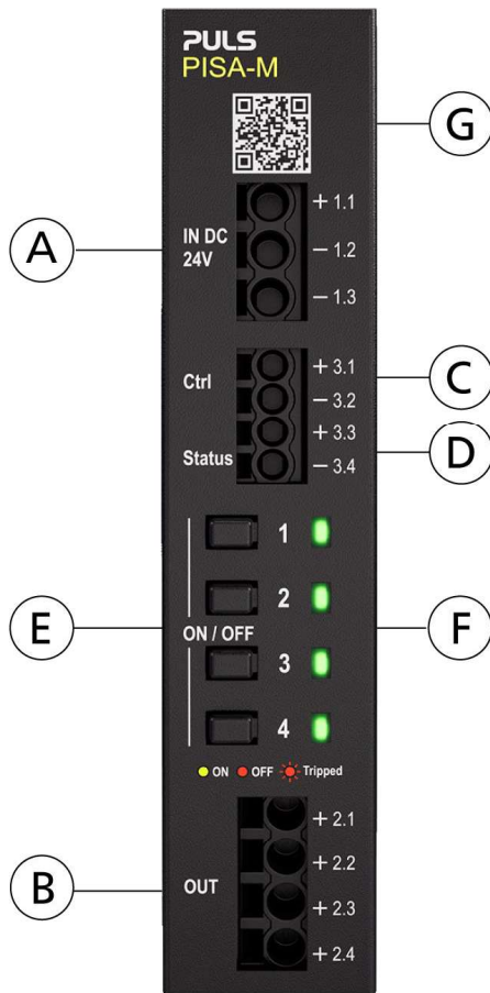
Fig. 14-1: Front side
