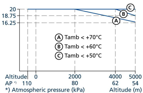
Fig. 20-2: Output current vs. altitude
