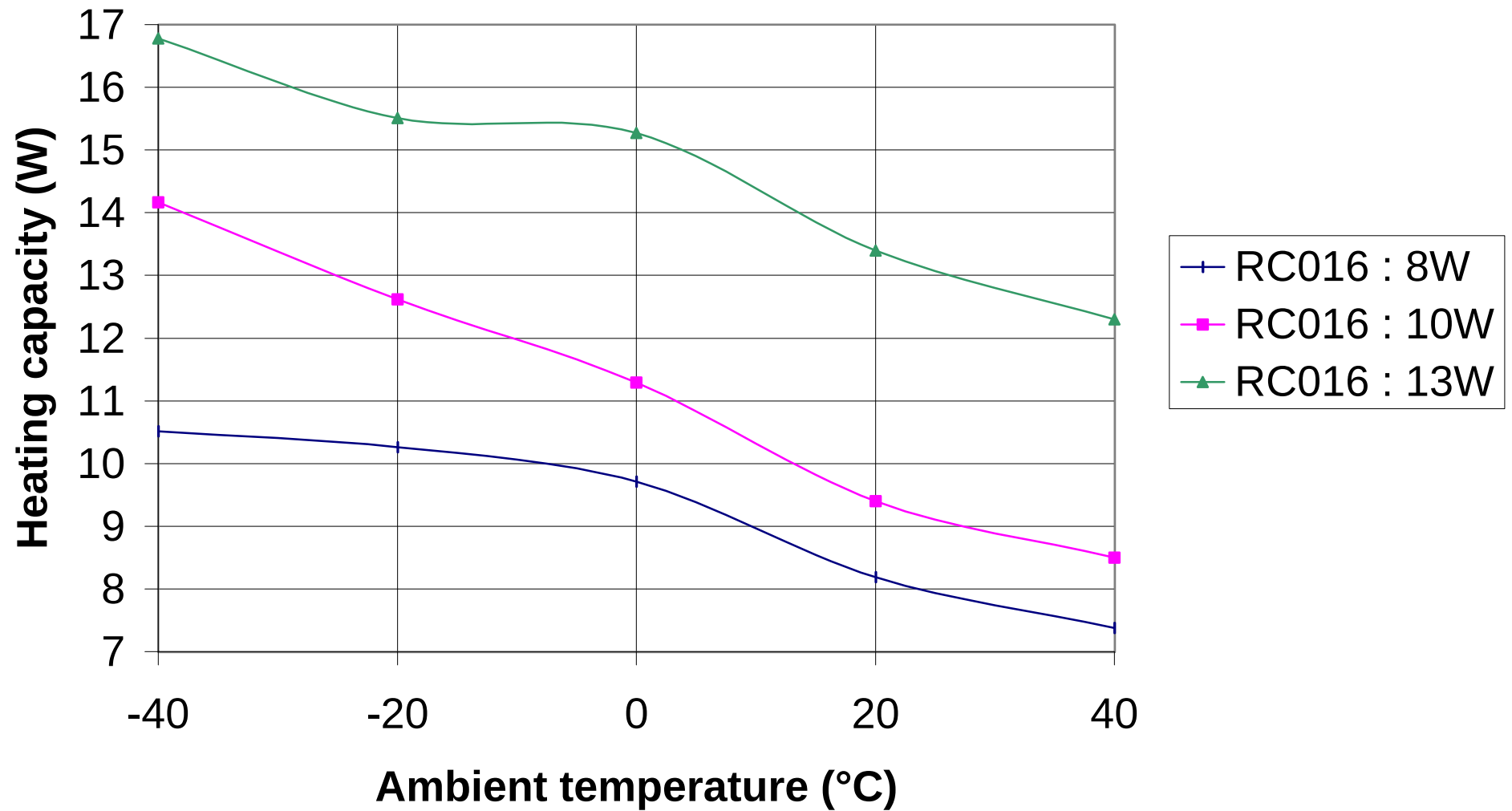
Heating capacity / Ambient temperature diagram
