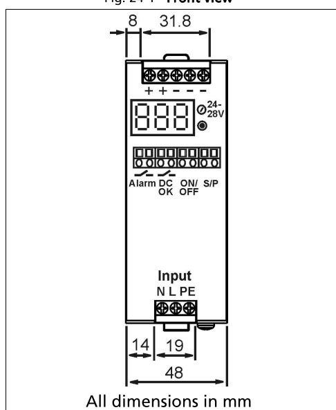
Fig. 24-1 Front view
