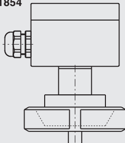
Threaded pipe connection per DIN 11854
