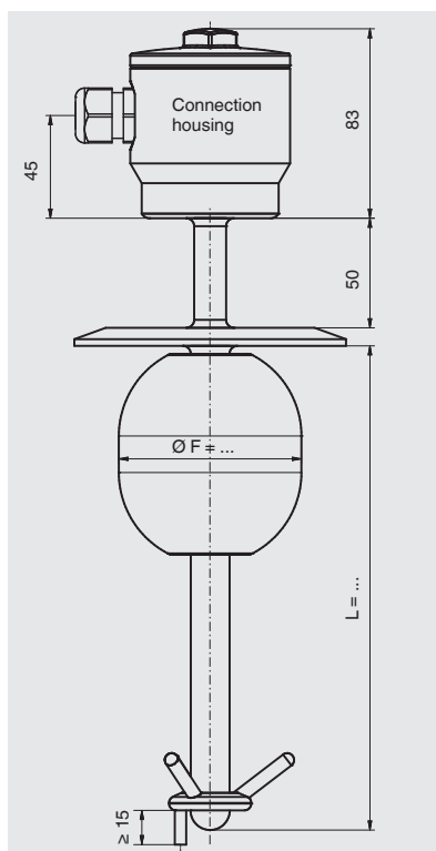
With welded tube end
