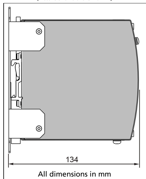
Fig. 23-6 Wall/panel mounting, side view (Picture shows the CP20.241)
