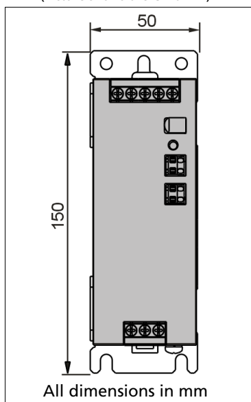
Fig. 23-4 Wall/panel mounting, front view (Picture shows the CP20.241)
