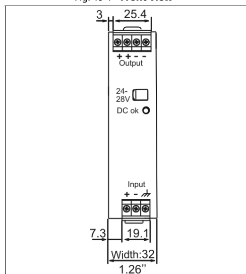
Fig. 19-1 Front view
