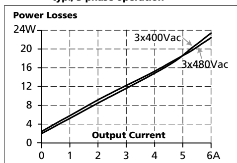
Fig. 8-2 Losses vs. output current at 48V, typ., 3-phase operation
